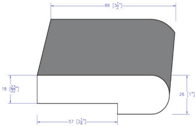
Stair Nose
