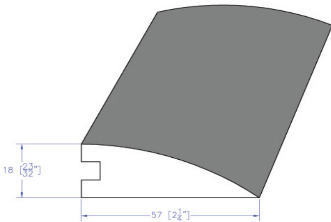
Reducer
