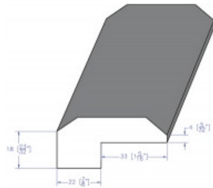
Carpet Reducer
