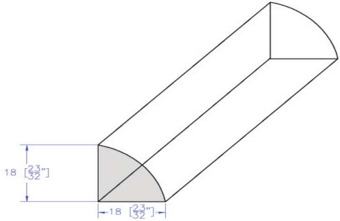
Base Shoe
