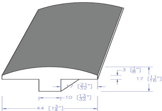
Transition Strip
